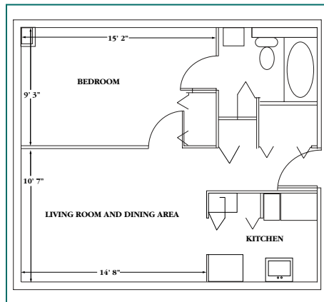
Below: Floor plan of a typical 460-square-foot apartment.
