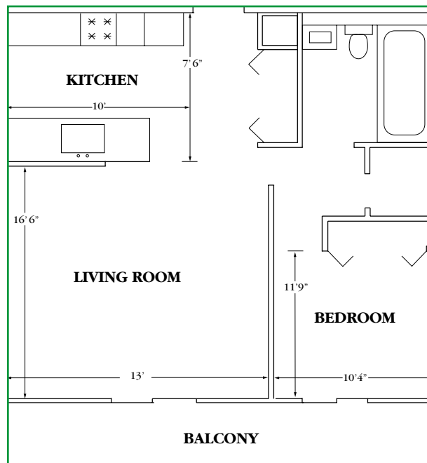
Floor plan of a typical 560-square-foot apartment.
